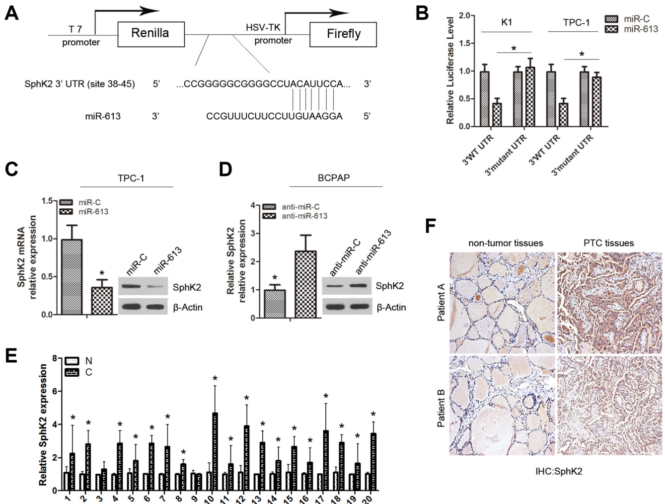
Figure 4: SphK2 is a direct target of miR-613. (A) Putative binding site of miR-613 in the SphK2 3'-UTR predicted by Target Scan. (B) Dual-luciferase activity of WT and mutant SphK2 3'-UTR reporter constructs in the presence of miR-613, relative to miR-C. (C) Expression of SphK2 was detected in TPC-1 cells transfected with miR-613 mimics or miR-C using qRT-PCR and western blots. (D) Expression of SphK2 was measured in BCPAP cells transfected with anti-miR-613 or anti-miR-C using qRT-PCR and western blots. (E) Expression of SphK2 was examined in PTC tissues (C) compared with non tumor tissues (N) by qRT-PCR. (F) Expression of SphK2 was analyzed using immunohistochemistry. * P < 0.05 .
