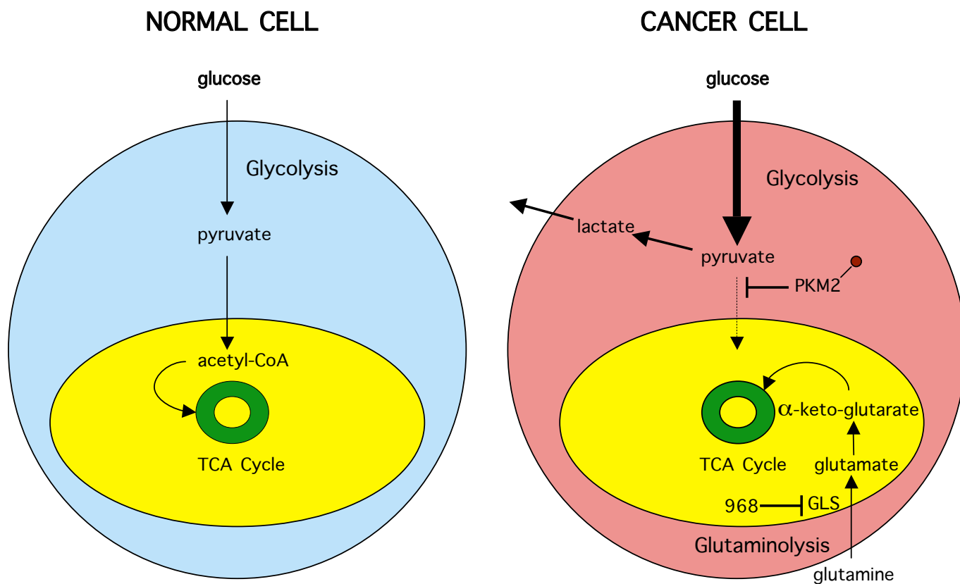
Figure 1: Metabolic remodeling of cancer cells Schematic highlights key differences in many cancer cells compared to normal tissue. Normal cells use glycolysis prior to respiration in the mitochondria (yellow) and complete breakdown of glucose by the tricarboxylic acid (TCA) cycle (green). In cancer cells, glycolysis becomes the primary mode of glucose metabolism resulting in lactate and its secretion. The M2 isoform of pyruvate kinase (PKM2) becomes tyrosine phosphorylated and attenuates pyruvate acetyl-CoA conversion while glutaminolysis provides the cancer cell with an alternate source of biosynthetic precursors, fueling the TCA cycle with glutamine-derived \alpha -keto-glutarate. The anti-tumor drug 968 inhibits glutamine metabolism by inhibiting the enzyme glutaminase (GLS).
