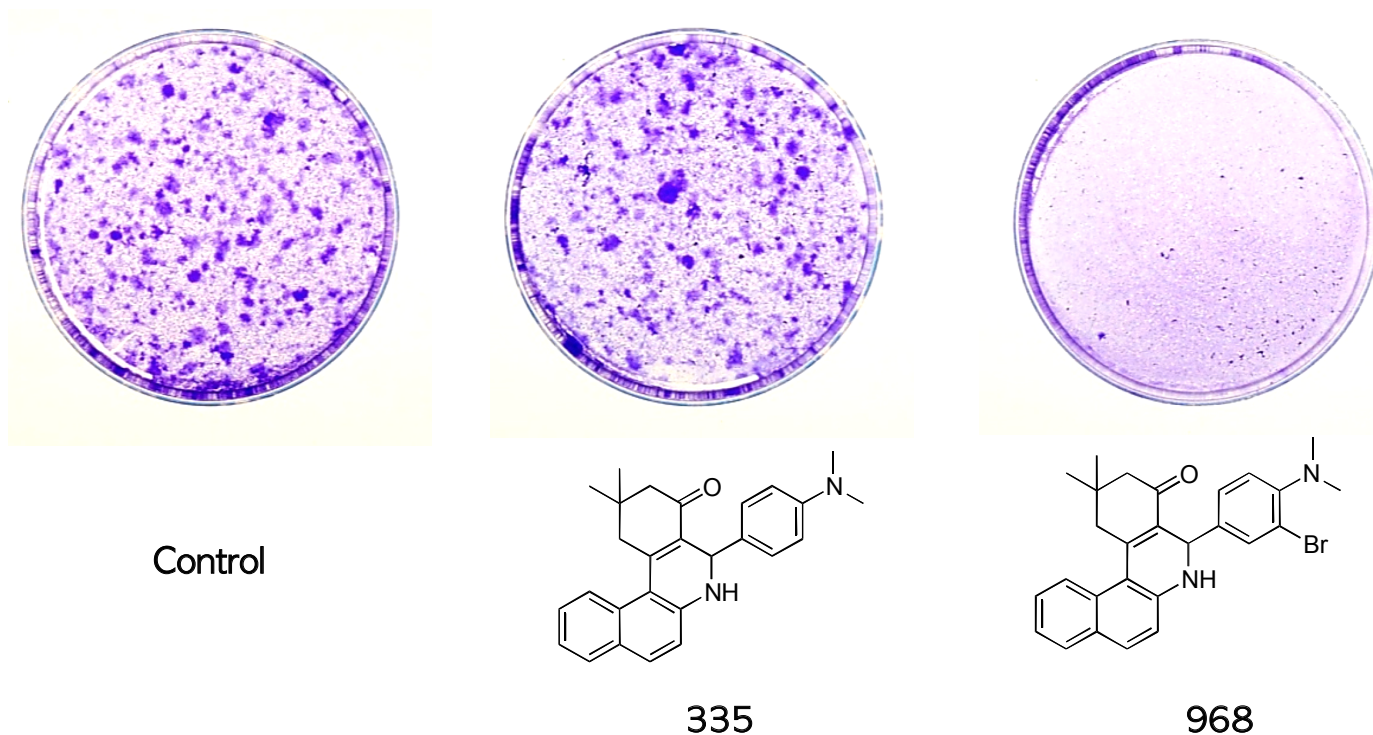
Figure 2: Glutaminase inhibition prevents Rho GTPase driven transformation. NIH-3T3 mouse fibroblasts in 10 cm plates were transfected with pZIPneoDbl and allowed to grow for 10 days in the presence of DMSO only (control), 5 \mu\text{M} of the inactive 968 analog 335 (CAS registry number 22949-42-4), or 5 \mu\text{M} 968 (CAS registry number 311795-38-7), after which the plates were fixed and stained with crystal violet. Structures of the inactive and active compounds are shown below treated cell samples.
