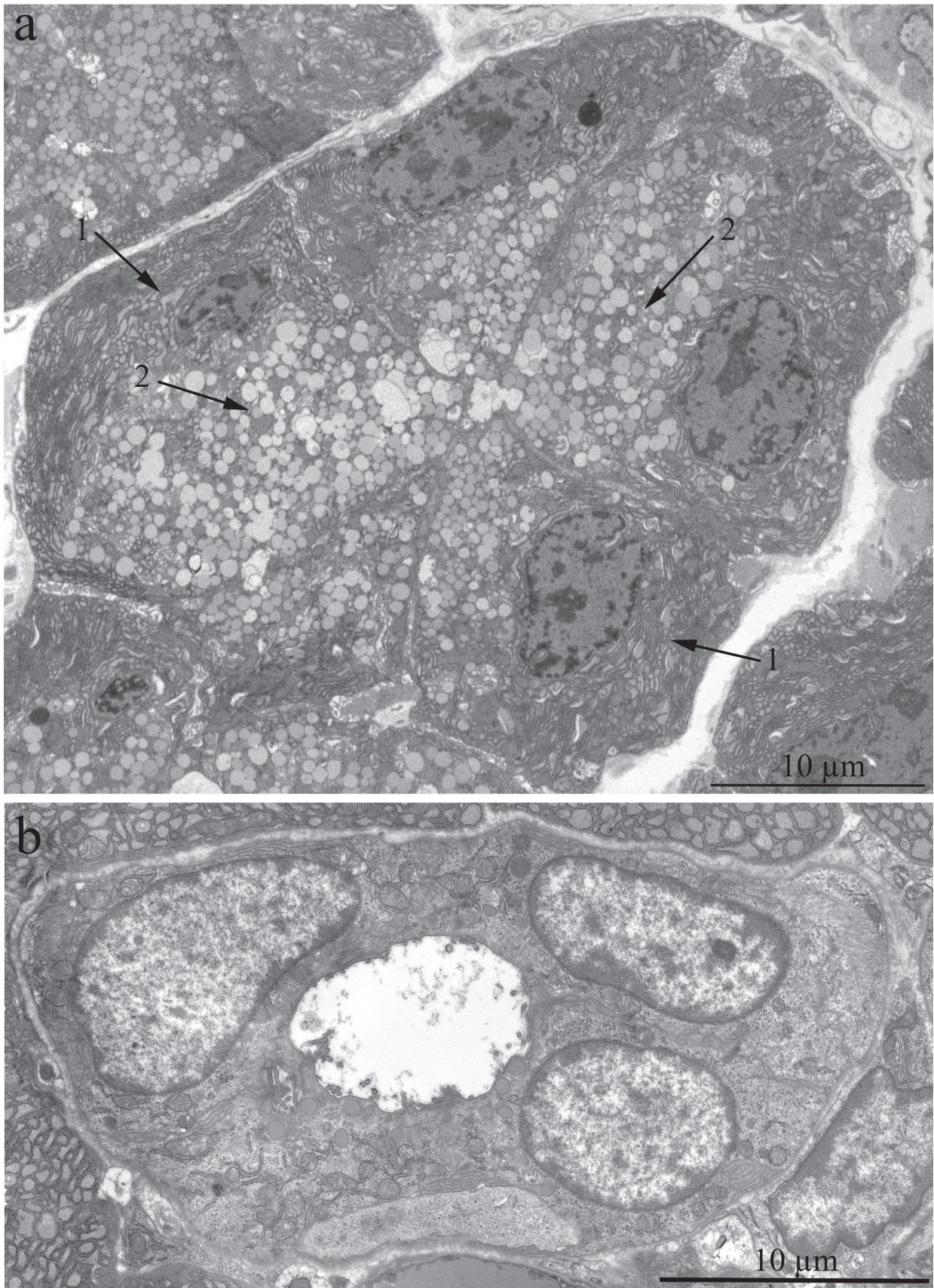
Figure 1: Ultrastructure of the lacrimal gland of Wistar rats at age 3 months. A. The rosette of acinar cells: acini. Arrows “1” indicate the ER; arrows “2” indicate secretory granules in acinar cells; B. The ultrastructure of an intercalary duct.
