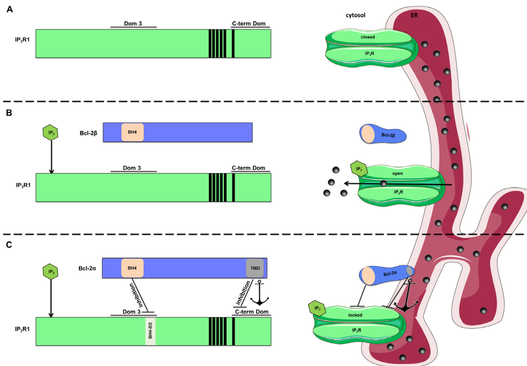
Figure 9: Model for inhibition of IP 3 R s by Bcl-2 proteins. The left side of the picture shows linear representation of the multi-domain interaction between Bcl-2 proteins and IP 3 R. On the right side these interactions are depicted within the ER membrane environment. A. Without IP 3 present, IP 3 R is in closed conformation and no Ca 2+ release occurs. B. Upon stimulation, IP 3 binds to the N-terminal ligand-binding domain of IP 3 R and leads to change in the conformation of the channel from closed to open state. This results in IP 3 R-mediated Ca 2+ release. Bcl-2 \beta , which similarly to our Bcl-2 ΔC , contains the BH4 domain, but lacks the TMD, might result in ineffective binding and regulation of the channel in cellulo . C. Efficient IP 3 R inhibition by Bcl-2 \alpha in cellulo requires multi-domain interaction between the two proteins, which involves binding of the BH4 domain of Bcl-2 \alpha to the Dom 3 of IP 3 R and binding between their C-termini. Here, we hypothesize that due to this multi-domain interaction, the IP 3 R is “locked” in a rigid conformation, leading to decreased Ca 2+ release through the channel even in presence of IP 3 . We propose a model, in which the interaction between the TMD of Bcl-2 \alpha and the C-term Dom of IP 3 R can “concentrate” the BH4 domain in the proximity of the Dom 3 by serving as an anchoring mechanism (indicated with an anchor). This “concentration effect” could overcome the inherent low affinity of inhibition by the BH4 domain. In addition to its anchoring role, the TMD of Bcl-2 \alpha has an inhibitory effect by itself.
