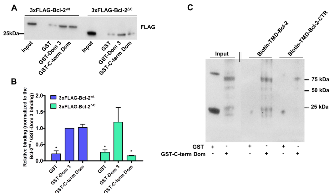
Figure 5: Bcl-2 requires its TMD for binding to the C-term Dom, but not to the Dom 3 of IP 3 R1. A. Representative GST-pull down experiments to compare the binding properties of 3xFLAG-Bcl-2 wt versus 3xFLAG-Bcl-2 ΔC overexpressed in COS-1 cells for GST-Dom 3 and GST-C-term Dom are shown. The binding to GST is used as a negative control. 0.1 μg of total COS-1 lysates was used as input. B. The immunoreactive bands from 4 independent experiments, utilizing each time independently transfected cells and freshly prepared lysates, were quantified and normalized to the binding of 3xFLAG-Bcl-2 wt to GST-Dom 3, which was set as 1. The data are plotted as mean ± S.E.M. C. Representative biotin pull-down experiment to study the binding of biotin-TMD-Bcl-2 or biotin-TMD-Bcl-2-CTR peptide to the purified GST or GST-C-term Dom is shown. The immunoblots were stained for GST. The experiment was performed 3 times. 0.2 μg of purified GST and GST-C-term Dom was loaded as input. The double line indicates that two parts of the same immunoblot and exposure time were merged together.
