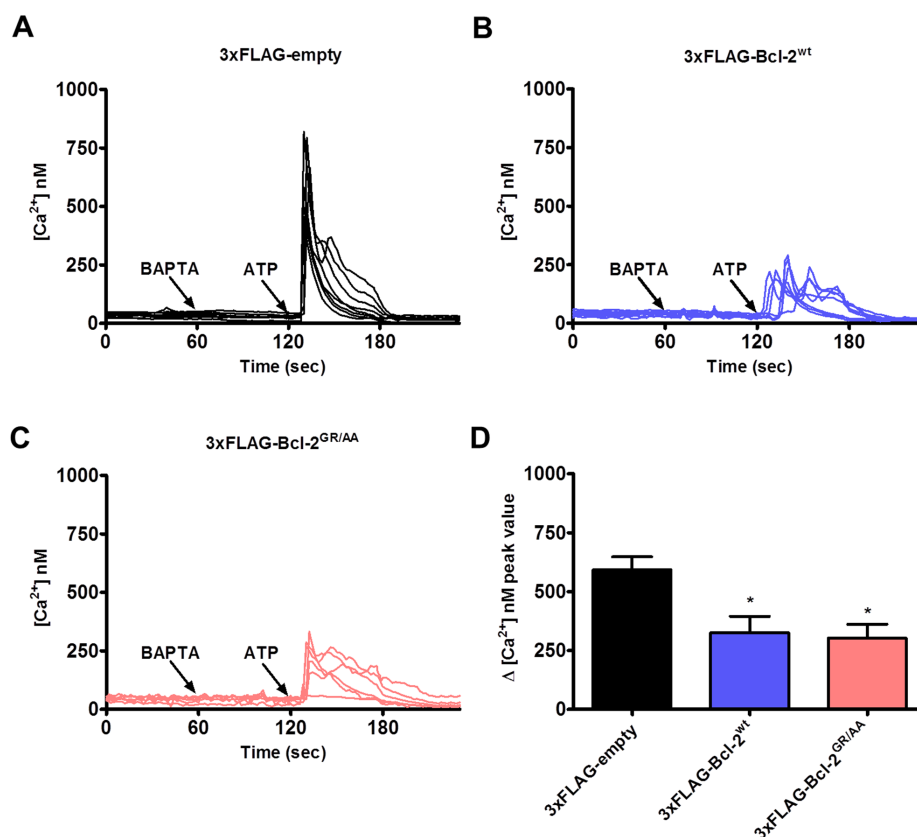
Figure 3: Bcl-2 GR/AA remains capable of inhibiting agonist-induced \text{Ca}^{2+} release. A-C. Intracellular \text{Ca}^{2+} release in response to 0.5 \mu\text{M} ATP was followed in the mCherry-positive Fura-2-AM loaded COS-1 cells overexpressing 3xFLAG-empty vector (A), 3xFLAG-Bcl-2 wt (B) or 3xFLAG-Bcl-2 GR/AA (C). The free extracellular \text{Ca}^{2+} was buffered by addition of 3 mM BAPTA. The obtained Fura-2 fluorescence signals (F340/F380) were calibrated and representative traces are plotted as [\text{Ca}^{2+}] . D. Quantitative analysis of the amplitude of the ATP-induced \text{Ca}^{2+} signals from at least 3 independent experiments ( n > 80 cells) is plotted as mean \pm S.E.M.
