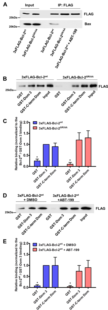
Figure 2: Bcl-2 GR/AA and Bcl-2 wt exposed to ABT-199 fail to bind pro-apoptotic Bax, but remain capable of binding the Dom 3 and the C-term Dom of IP 3 R. A. Representative FLAG-co-immunoprecipitation experiment for detection of the 3xFLAG-Bcl-2/Bax interaction is shown. Overexpressed 3xFLAG-Bcl-2 wt (in absence and presence of 3 \mu M ABT-199) or 3xFLAG-Bcl-2 GR/AA was immunoprecipitated from COS-1 cell lysates by anti-FLAG-loaded agarose beads. The immunoreactive blots were stained with antibody against FLAG and Bax. 0.1 \mu g and 0.5 \mu g of total COS-1 lysates were used as input for the 3xFLAG-proteins and Bax respectively. The experiments were performed 3 times utilizing each time independently transfected cells and freshly prepared lysates. B. Representative GST-pull down experiments with COS-1 cell lysates for comparing the binding of overexpressed 3xFLAG-Bcl-2 wt and 3xFLAG-Bcl-2 GR/AA to the GST-Dom 3 and GST-C-term Dom are shown. The samples were analyzed via Western blot and stained with anti-FLAG antibody. The binding to the GST was used as a negative control. 0.1 \mu g of total COS-1 lysates was used as input. C. The immunoreactive bands from 3 independent experiments, utilizing each time independently transfected cells and freshly prepared lysates, were quantified and normalized to the binding of 3xFLAG-Bcl-2 wt to GST-Dom 3, which was set as 1. The data are plotted as mean \pm S.E.M. D. Representative GST-pull down experiments with COS-1 cell lysates for comparing the binding of overexpressed 3xFLAG-Bcl-2 wt in absence and presence of 3 \mu M ABT-199 to the GST-Dom 3 and GST-C-term Dom are shown. The samples were analyzed via Western blot and stained with anti-FLAG antibody. The binding to the GST was used as a negative control. 0.1 \mu g of total COS-1 lysates was used as input. E. The immunoreactive bands from 3 independent experiments, utilizing each time independently transfected cells and freshly prepared lysates, were quantified and normalized to the binding of 3xFLAG-Bcl-2 wt to GST-Dom 3, which was set as 1. The data are plotted as mean \pm S.E.M.
