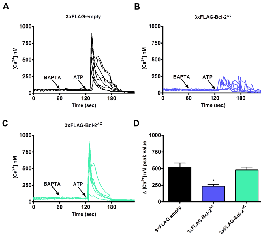
Figure 6: Bcl-2 ΔC fails to inhibit IP 3 R-mediated Ca 2+ release. A-C. Intracellular Ca 2+ release in response to 0.5 μM ATP was followed in the mCherry-positive Fura-2-AM loaded COS-1 cells overexpressing 3xFLAG-empty vector (A), 3xFLAG-Bcl-2 wt (B) or 3xFLAG-Bcl-2 ΔC (C). The free extracellular Ca 2+ was buffered by addition of 3 mM BAPTA. The obtained Fura-2 signals (F340/F380) were calibrated and representative traces are plotted as [Ca 2+ ]. D. Quantitative analysis of the amplitude of the ATP-induced Ca 2+ signals from 5 independent experiments (n > 110 cells) is plotted as mean ± S.E.M.
