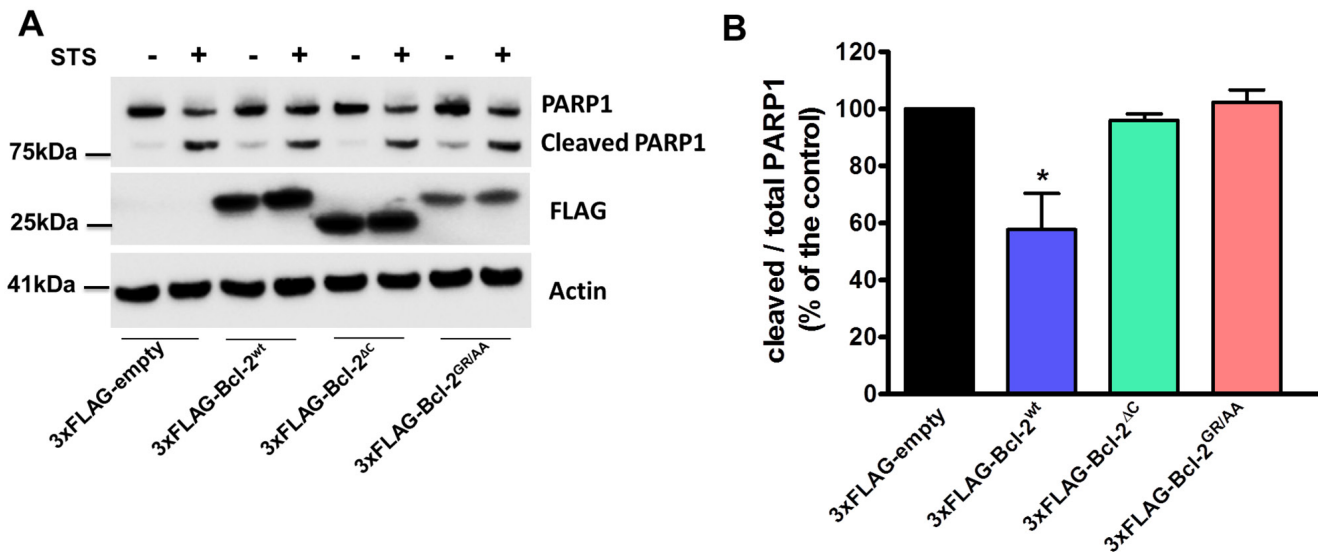
Figure 8: The TMD of Bcl-2 is required for STS-induced apoptosis. A. Western-blot analysis for monitoring PARP1 cleavage upon staurosporine (STS) treatment (1 \mu M for 6 h) in COS-1 cells overexpressing 3xFLAG-empty, 3xFLAG-Bcl-2 wt , 3xFLAG-Bcl-2 GR/AA or 3xFLAG-Bcl-2 ΔC . 7 \mu g of total cell lysate were loaded and the immunoblots were stained for PARP1, FLAG and Actin. B. Quantification of the ratio of the immunoreactive bands of cleaved over full-length PARP1 from 4 independent experiments, utilizing each time independently transfected COS-1 cells and freshly prepared lysates. The ratio of cleaved over full-length PARP1 obtained for control cells was set as 100% and the other ratios were normalized to this value. The data are plotted as \pm S.E.M.
