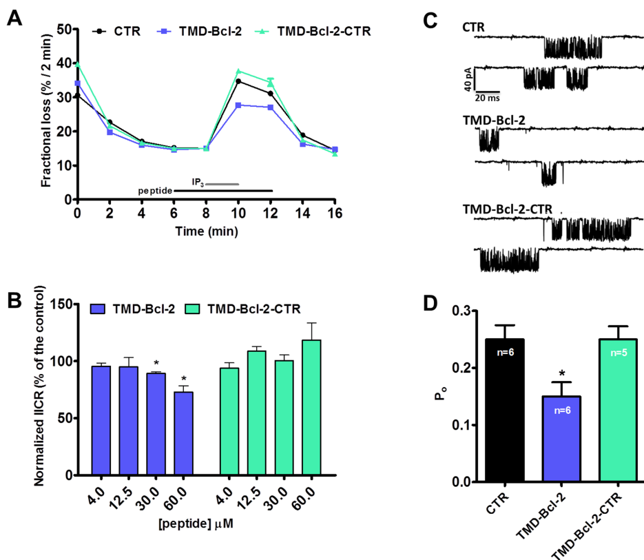
Figure 7: The TMD of Bcl-2 is sufficient to inhibit IP_3R s in permeabilized cell systems and single-channel recordings. A. Typical experiment of unidirectional ^{45}Ca^{2+} fluxes in permeabilized MEFs. Ca^{2+} release was induced by 3 \mu M IP_3 (grey bar) in control condition or in presence of 60 \mu M peptides, TMD-Bcl-2 or TMD-Bcl-2-CTR (black bar). The results are plotted as fractional loss after 2 min of incubation with IP_3 minus the fractional loss before the addition of IP_3 (%/2 min) as a function of time. B. Quantification of the IICR from 5 independent experiments. The values of IICR measured as fractional loss were calculated as percentage of the IICR in control condition, which was set as 100%. C. Representative IP_3R1 single-channel recordings from DT40 cells ectopically expressing IP_3R1 evoked by 1 \mu M IP_3 at 200 nM Ca^{2+} and 5 mM ATP, in control condition or in presence of the TMD-Bcl-2 or TMD-Bcl-2-CTR peptides. D. Histogram depicting the open probability ( P_o ) \pm SD for the IP_3R1 under the previously described conditions. The total number of recordings for each condition is indicated within every bar.
