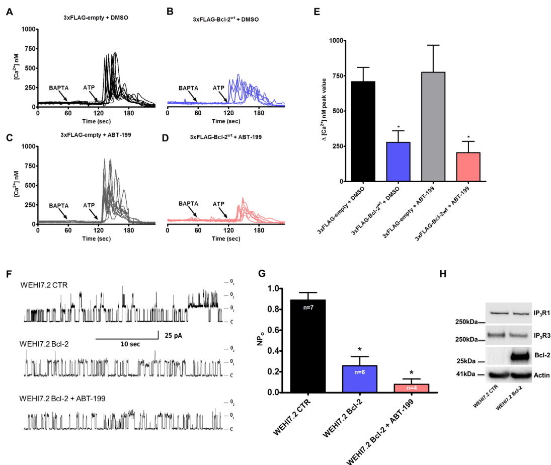
Figure 4: ABT-199 does not impact Bcl-2's ability to suppress IP 3 R activity in single-cell measurements and in patch-clamp single-channel recordings. A-D. Intracellular Ca 2+ release in response to 0.5 \mu M ATP was followed in the mCherry-positive Fura-2-AM loaded COS-1 cells overexpressing 3xFLAG-empty vector (A, C) or 3xFLAG-Bcl-2 wt (B, D) in absence (A, B) or presence of 3 \mu M ABT-199 (C, D). The free extracellular Ca 2+ was buffered by addition of 3 mM BAPTA. The obtained Fura-2 fluorescence signals (F340/F380) were calibrated and representative traces are plotted as [Ca 2+ ] i . E. Quantitative analysis of the amplitude of ATP-induced Ca 2+ signals from at least 3 independent experiments (n > 80 cells) is plotted as mean \pm S.E.M. F. Representative IP 3 R currents in ER-containing membrane fractions from control (WEHI7.2 CTR) (top) and Bcl-2-expressing WEHI7.2 cells without (middle) or with (bottom) application of 1 \mu M ABT-199. The IP 3 R activity was triggered by 5 \mu M IP 3 and 1 \mu M Ca 2+ . G. The mean levels of IP 3 R activity (NP o ) under these conditions are summarized and the data are plotted as mean \pm S.E.M. The total number of recordings for each condition is indicated within every bar. H. Western blot analysis of the expression levels of Bcl-2, IP 3 R1 and IP 3 R3 in WEHI7.2 CTR and WEHI7.2 Bcl-2 cells. 5 \mu g of total lysate was loaded and the immunoreactive bands were stained against Bcl-2, IP 3 R1, IP 3 R3 and actin.
