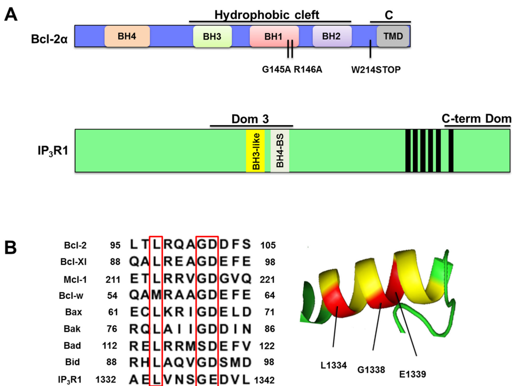
Figure 1: The Dom 3 of IP 3 R1 contains a BH3 motif. A. Linear representation of Bcl-2 and IP 3 R1. Bcl-2α is depicted in blue with its BH domains and the trans-membrane domain (TMD). The two functional domains of interest, the hydrophobic cleft formed by BH3-BH1-BH2 domains and the C-terminus (C), are indicated with black lines. The C-terminal region, containing the TMD, is present in Bcl-2α, but not in Bcl-2β. The G145 and R146 residues, located in the BH1 domain were mutated to yield Bcl-2 GR/AA . Bcl-2 was truncated at W214 residue to yield Bcl-2 AC , which correlates with Bcl-2β. A schematic representation of IP 3 R1 is depicted in green. The Bcl-2-binding fragments of IP 3 R used in this study, the domain 3 (Dom 3) and the C-terminal domain containing the last TMD (C-term Dom), are indicated with black lines and the six TMDs are shown as black bars. The exact BH4-binding site in the Dom 3 is represented in light grey (BH4-BS). The BH3-like motif in the Dom 3 is represented in yellow. B. The Dom 3 of IP 3 R1 contains a BH3 motif. Left: Sequence alignment between the BH3 domains of Bcl-2 family members and the Dom 3 of IP 3 R1 reveals the presence of the conserved residues (LxxxGD/E, pointed in red), required for a typical BH3 motif (46). Right: A secondary structure prediction of the putative BH3 motif of IP 3 R1 present in the Dom 3 sequence, predicted by the I-TASSER web server and drawn using PyMol. The predicted BH3 motif within the Dom 3 is depicted in yellow and the conserved residues in red.
